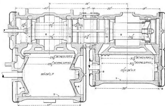
Fig. 2208. Arrangement of Cylinders and Valves of Cole Four-Cylinder Balanced Compound Locomotive. American Locomotive Co.
